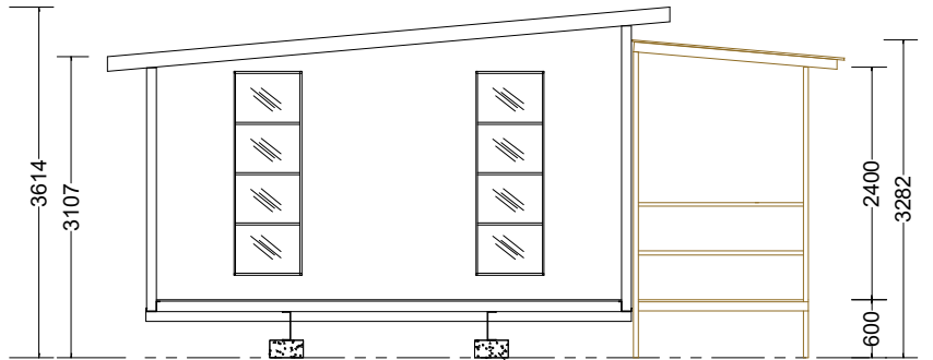
Left Elevation
